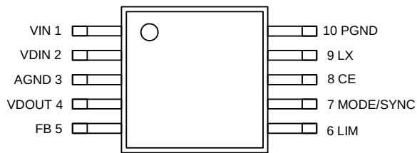
MSOP-10 (TOP VIEW)
