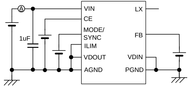
Circuit ②
