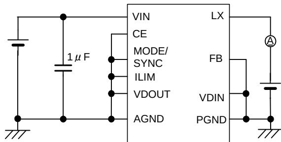
Circuit ⑥
