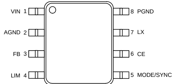
SOP-8 (TOP VIEW)
