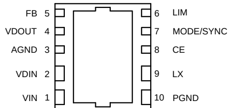
USP-10B (BOTTOM VIEW)
