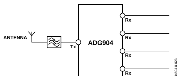
Figure 29. Tx/Rx Switching
