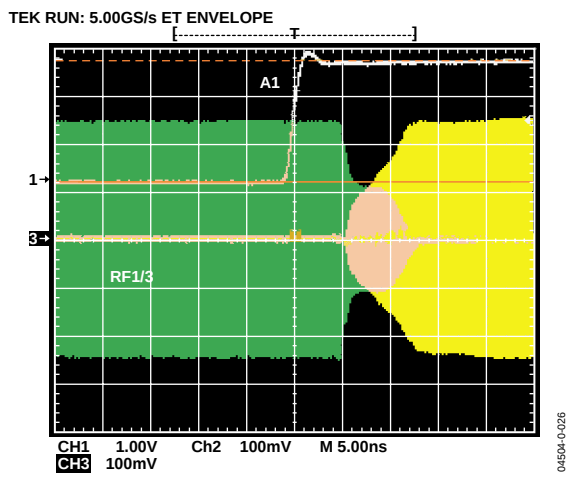
Figure 15. Switch Timing
