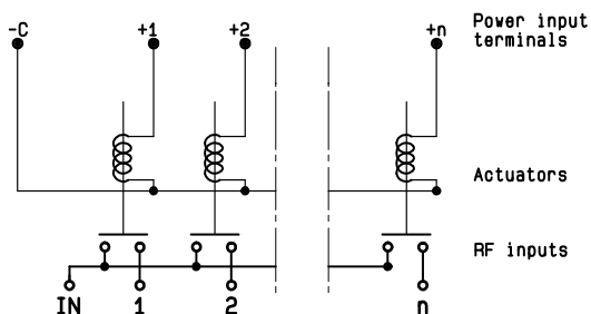
NORMALLY OPEN WITHOUT OPTION R591 -0- -0-
