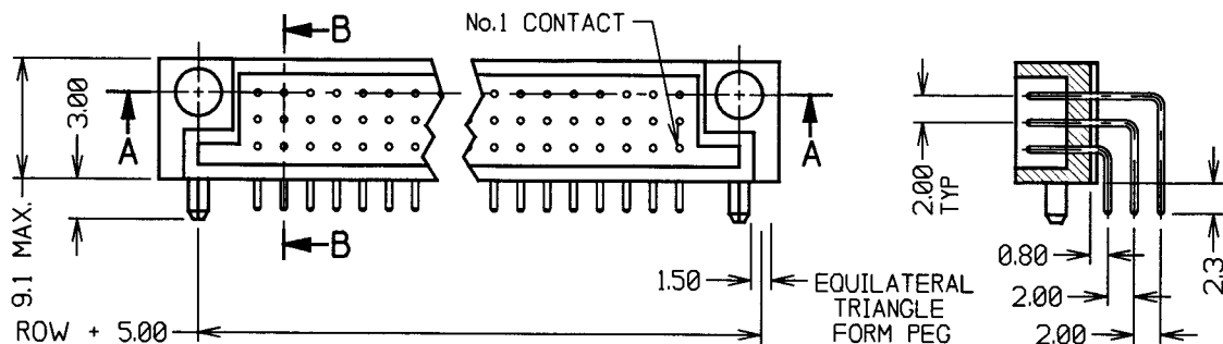
SECTION B-B
