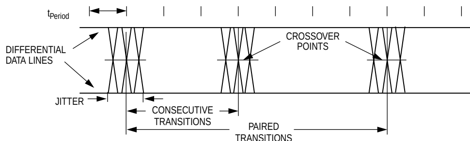
Figure 9-12. Data Jitter
