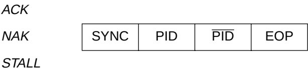
Figure 9-3. Supported USB Packet Types
