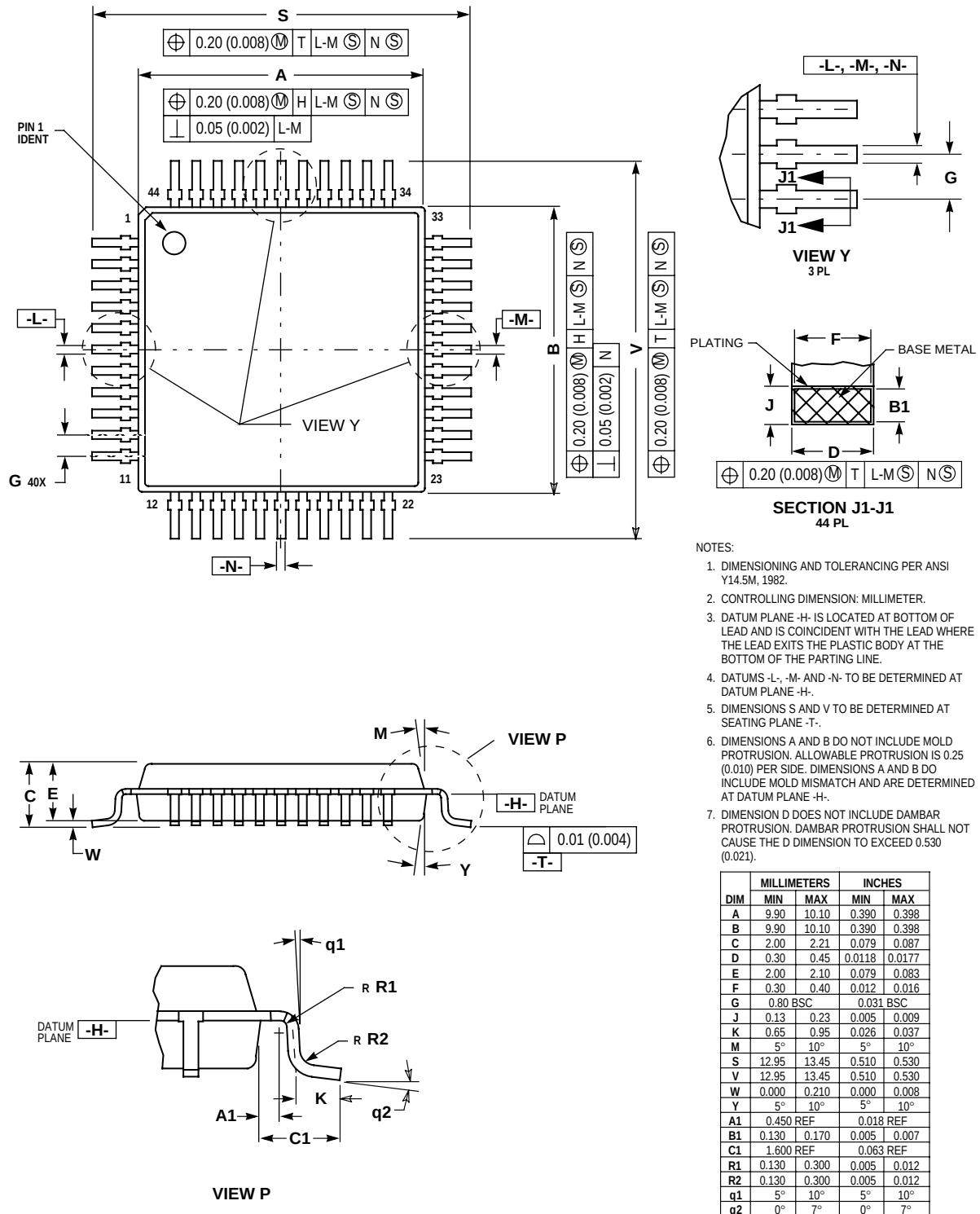
Figure 19-3. 44-Pin QFP (Case #824E)
