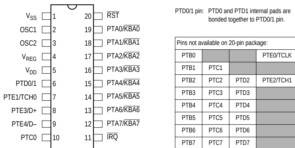
Figure 1-4. 20-pin PDIP Pin Assignments
